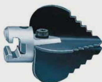
RIDGID T26 4 BLADE CUTTER 4.5" 680257
